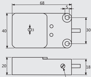
可调旋钮 Adjustable knob 灵敏度调节 sensitivity modulation
